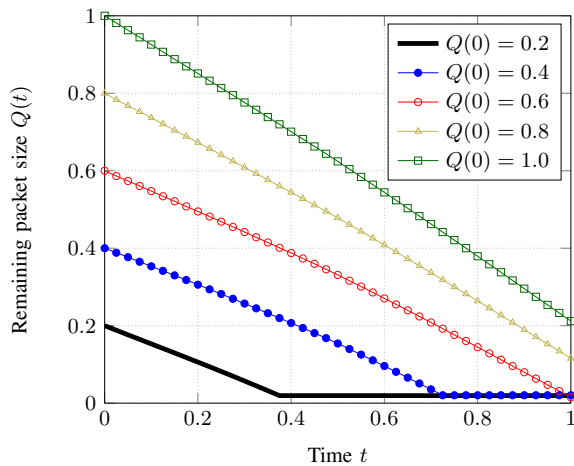
Fig. 2. Remaining packet size Q(t) under optimal power p^*(t, Q_t) for users with initial packet size Q(0) \in \{0.2, 0.4, 0.6, 0.8, 1\} .
